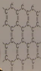
Graphit/Graphen
